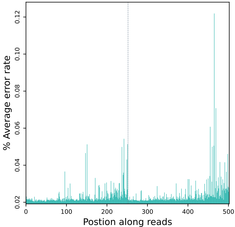
Error rate distribution along reads (R10813)
